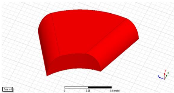
Fig. 5. Improved PM shape.
