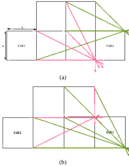
Fig. 3 (a): Forces on the electrons of cell 2 in state1, (b) Forces on the electrons of cell 2 in state2.
