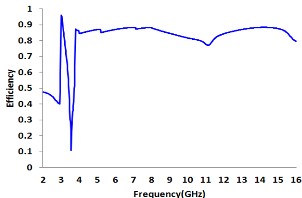
Fig. 3. The antenna efficiency (simulation result).
