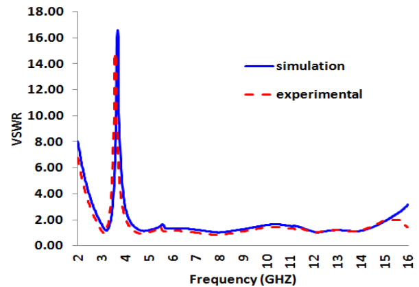
Fig.2. Simulation and experimental results of the VSWR.
