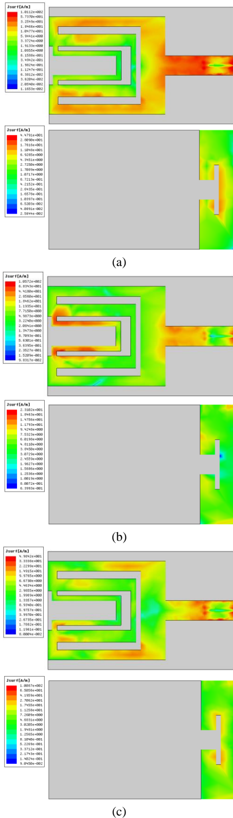
Fig. 6. The surface current distribution at (a) 2GHz, (b) 6 GHz, and (c) 10 GHz.
