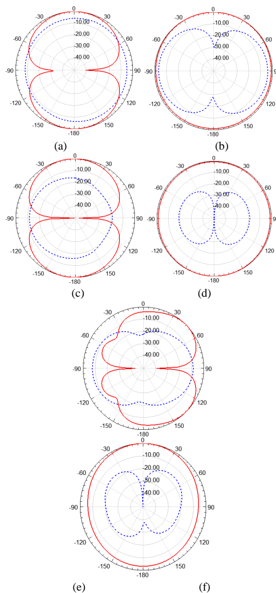
Fig. 5. Simulated radiation patterns of the proposed antenna (solid line for co-polarization and dash line for cross polarization), (a) E-plane at 2.8 GHz, (b) H-plane at 2.8 GHz, (c) E-plane at 6 GHz, (d) H-plane at 6 GHz, (e) E-plane at 10 GHz, (f) H-plane at 10 GHz
