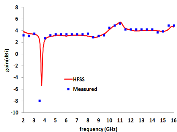
Fig. 4. The simulated and measured antenna gain.
