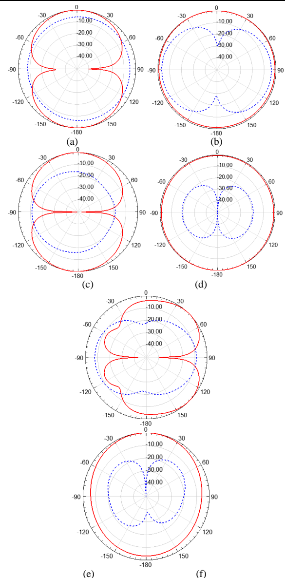
Fig. 5. Simulated radiation patterns of the proposed antenna (solid line for co-polarization and dash line for cross polarization)
