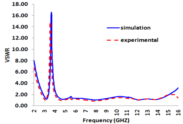
Fig.2. Simulation and experimental results of the VSWR.
