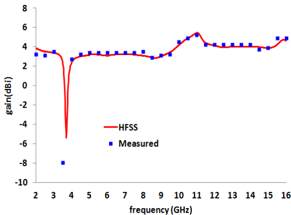
Fig. 4. The simulated and measured antenna gain.
