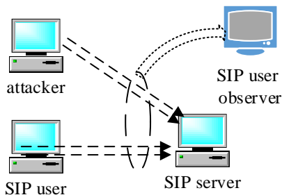
Fig. 3. Simulation testbed.
