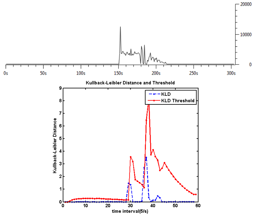
Fig. 6. Attack detection with traffic rate of 10 calls per second and attack mass of 1000000 INVITE messages.
