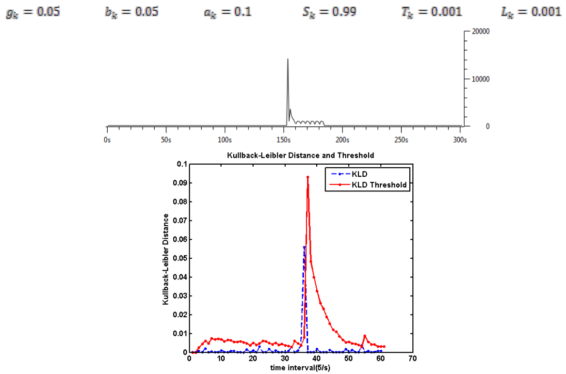
Fig. 10. Attack detection with traffic rate of 100 calls per second and attack mass of 10000 INVITE messages.
