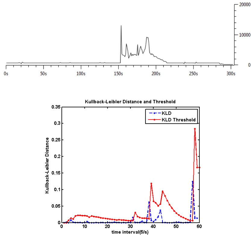
Fig. 12. Attack detection with traffic rate of 100 calls per second and attack mass of 100000 INVITE messages.
