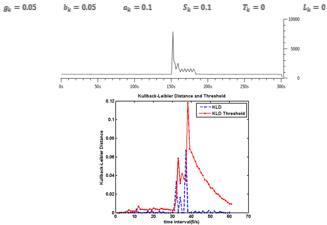
Fig. 11. Attack detection with traffic rate of 100 calls per second and attack mass of 100000 INVITE messages.
