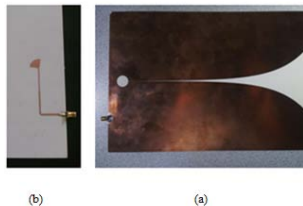
Fig. 4 (a) Fabricated Vivaldi antenna by Butterworth method (b) Feed line of antenna.
