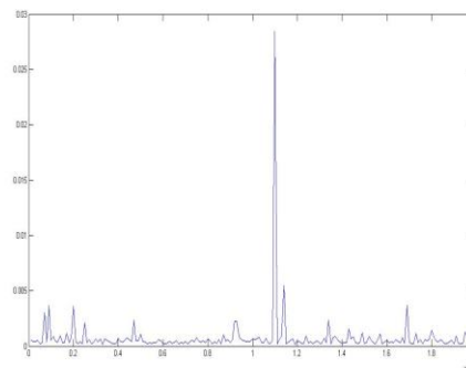
Fig. 14. The maximum amplitude of PD in the case of DC voltages in oil-impregnated paper testing object
